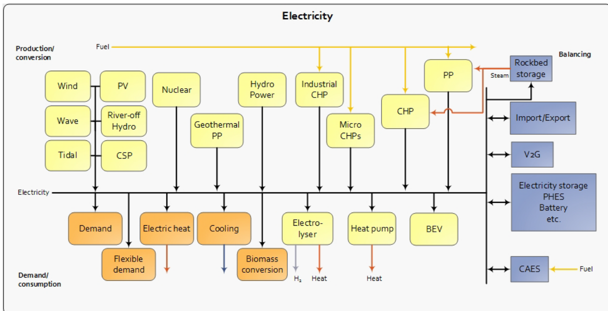
Illustration of components involved when the EnergyPLAN model calculates hourly balancing of the ELECTRICITY system including interactions with other parts of the whole system
