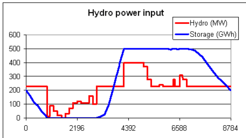
Diagram 6.5: Hydro power output with limitations on water storage capacity
